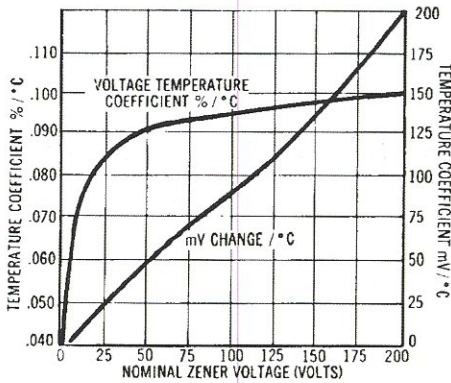
FIGURE 2 ZENER VOLTAGE TEMPERATURE COEFF. vs. ZENER VOLTAGE
